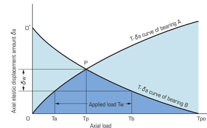
Figure 5.3 Fixed-position Preload
