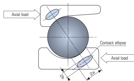
Figure 2.3 Contact Ellipse
