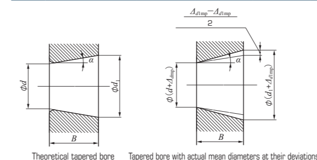
Figure 3.1 Tapered Bores of Cylindrical Roller Bearings
