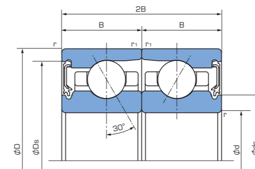
NKE (Non-contact seal)
