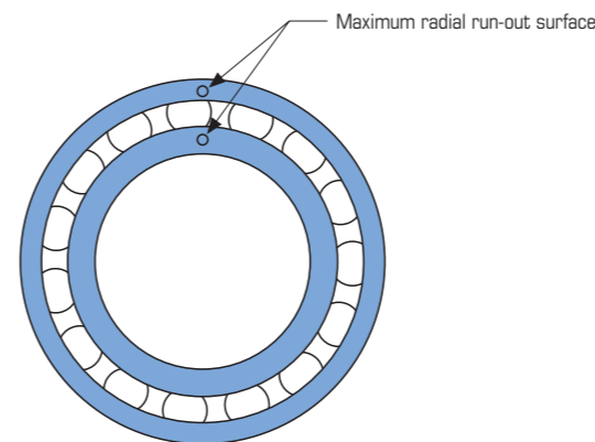
Figure 9.6 Maximum Radial Run-out Locations
