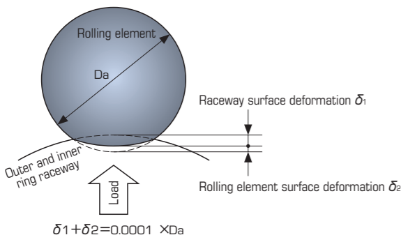
Figure 2.2 Permanent Indentation
